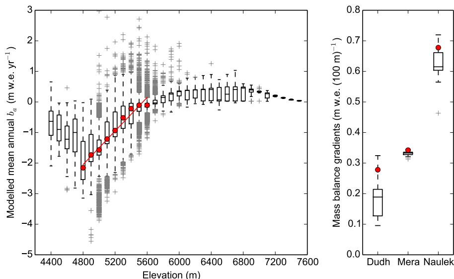
Figure 12. Left: boxplots of modelled mean annual mass balance (m w.e. yr -1 ) calculated for 100 m intervals (1961–2007) for the entire Dudh Koshi basin. Calculated mass balance gradient of 0.27 m w.e. (100 m) -1 between 4850 and 5650 m is shown in red. Right: boxplots of mass balance gradients calculated for all 20 calibration model runs for the entire Dudh Koshi (between 4850 and 5650 m), Mera Glacier (between 5350 and 5600 m), and Naulek Glacier (between 5350 and 5600 m). The gradients calculated for Run 5 are shown in red.
