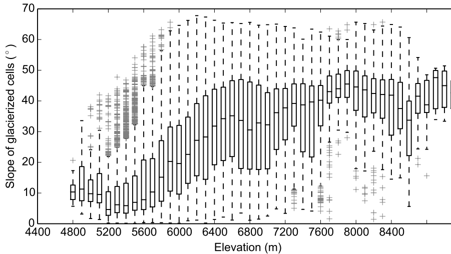
Figure 7. Boxplots of the slope of glacierized pixels in the Dudh Koshi basin, grouped by 100 m elevation bands. The boundaries of each box indicate the upper and lower quartiles, while the middle line of the box shows the median value. Whisker ends indicate the maximum (minimum) values excluding outliers, which are defined as more (less) than 3/2 times the upper (lower) quartile. Slope values were extracted from the SRTM 90 m DEM and glacier inventory from ICIMOD (2011).
