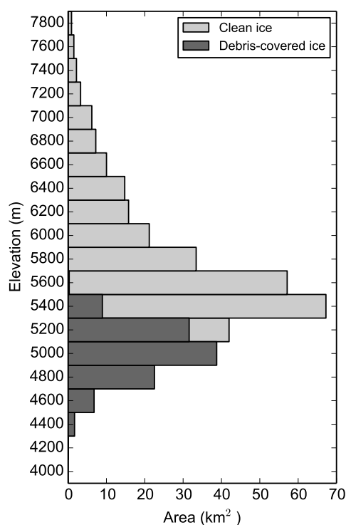
Figure 2. Area of clean and debris-covered glaciers by elevation, Dudh Koshi basin, Nepal. Extracted from SRTM 90 m DEM and glacier inventory from ICIMOD (2011)
