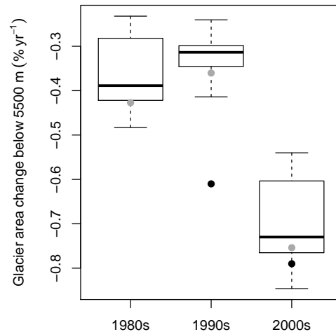
Figure 15. Rates of historical glacier area change below 5500 m ( \% \text{ yr}^{-1} ) from the 20 model runs. Remotely sensed rates of glacier area change and Run 5 results are shown as black and grey points, respectively. The 1980's inventory contained inaccuracies related to the resolution of the imagery and the misclassification of snow as glacier ice, and an observed rate of change from 1980 to 1990 is not included here.
