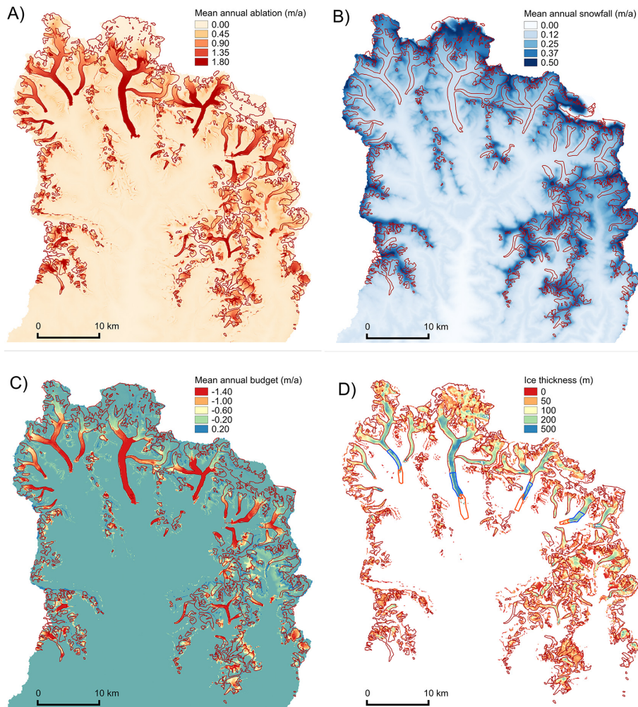
Figure 11. Results from the calibrated model run, 1961–2007. (a) Mean annual ablation, (b) mean annual snowfall, (c) mean annual mass budget, and (d) final ice thickness. Extents of glacierized and non-glacierized calibration regions are shown in (d).
