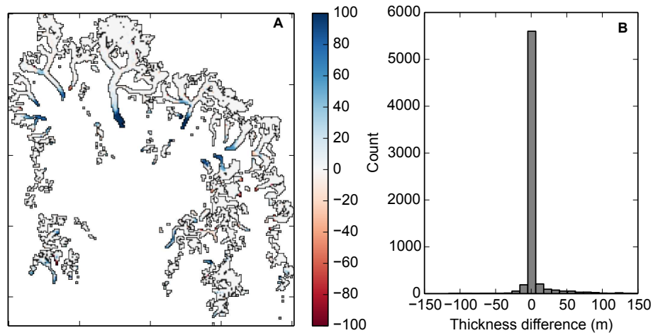
Figure 8. (a) Differences in modelled ice thickness (in m) between the end of the first initialization run (47 years) and after an additional 94 years of simulation with dT = -1.2 °C. (b) Histogram of differences in modelled ice thickness.
