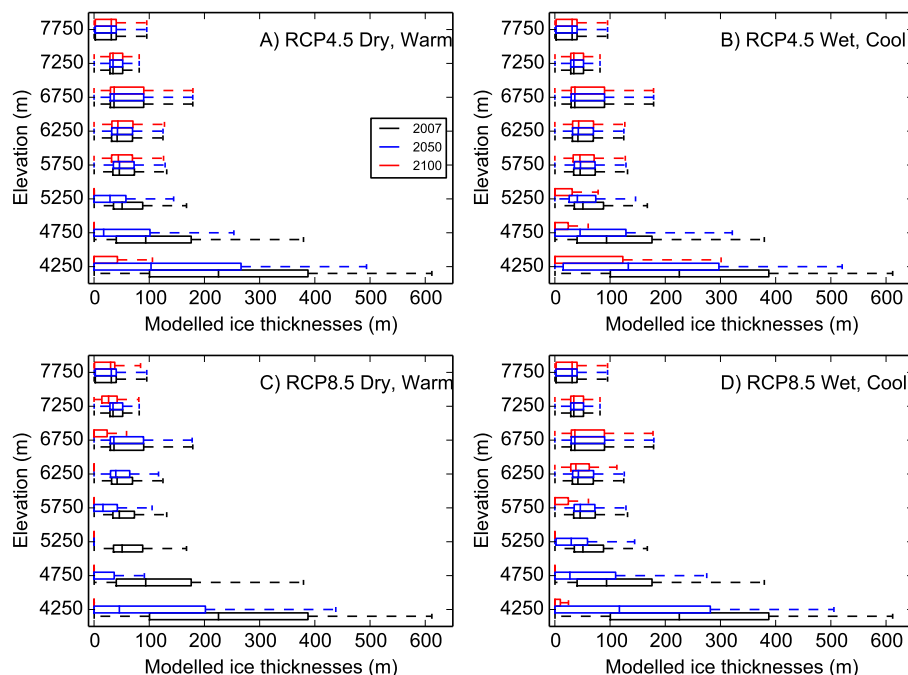
Figure 18. Distribution of modelled ice thicknesses by elevation band, for 2007 (initialization), 2050, and 2100. (a) Dry/warm RCP4.5 scenario, (b) , wet/cool RCP4.5 scenario, (c) dry/warm RCP8.5 scenario, and (d) wet/cool RCP8.5 scenario.
