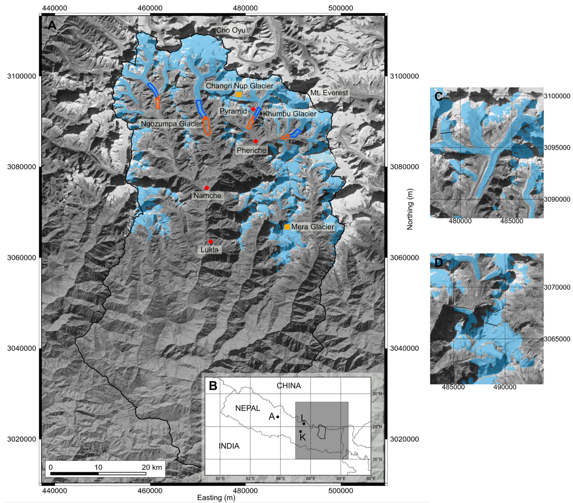
Figure 1. (a) Dudh Koshi basin, eastern Nepal, with current glacier extents in blue (ICIMOD, 2011), EVK2CNR stations (red), GPR profile sites (yellow). Extents of glacierized (blue) and non-glacierized (orange) regions used for model calibration are also shown. Coordinate system is UTM 45N. Inset map (b) shows the Dudh Koshi basin in relation to the APHRODITE subset (shaded), and the locations of places named in the text (A – Annapurna, L – Langtang, K – Kathmandu). Panels (c) and (d) give the location of the transverse GPR surveys (thick red lines) at Changri Nup and Mera glaciers, respectively.
