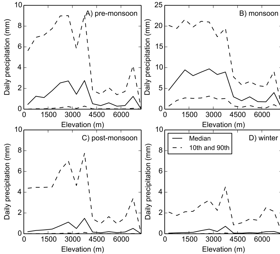
Figure 5. APHRODITE precipitation (1961–2007) binned by elevation for pre-monsoon (a), monsoon (b), post-monsoon (c), and winter (d). Median, 10th percentile, and 90th percentile of daily precipitation are shown. Note different scale for panel (b).
