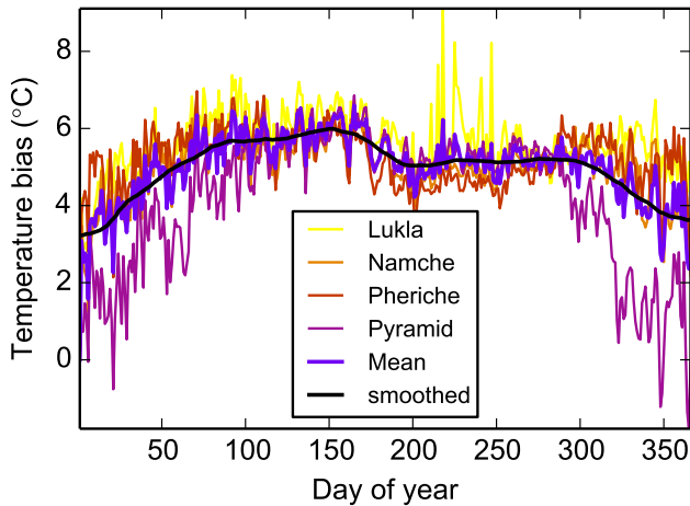
Figure 4. Average daily temperature bias (estimated – observed) for four EVK2CNR sites (2003–2007), their arithmetic mean, and a smoothed function used as a daily bias correction.
