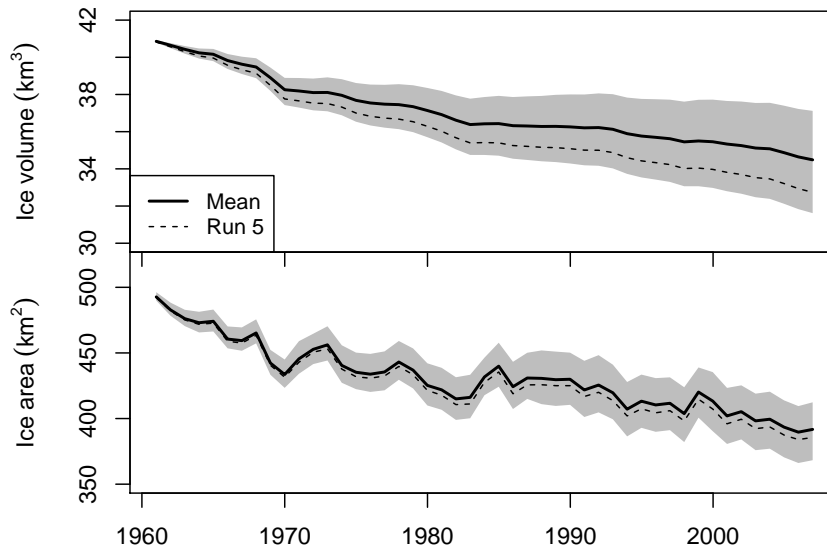
Figure 10. Top panel: modelled mean (1 November–31 January) ice volumes from the 20 calibration runs, 1961–2007, with multi-model mean (black line), minimum and maximum modelled volumes (shaded area), and results from Run 5 (dashed line). Bottom panel: as above but for modelled glacier areas from the 20 calibration runs.
